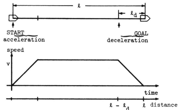
Fig. 7 Moving straight-1
