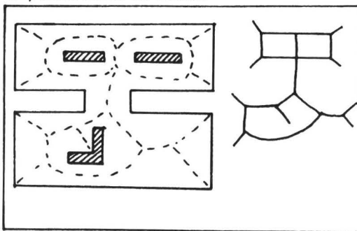
Figure 3. A skeletal graph and its corresponding path graph
