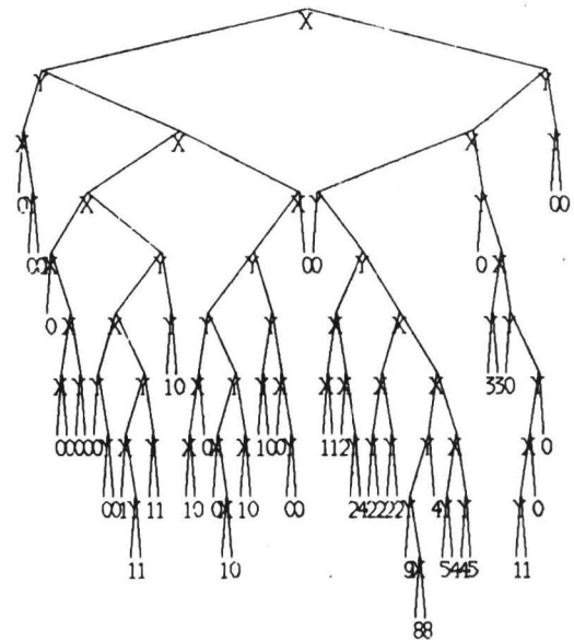
Figure 3. The tree structure of the DQ Space of Figure 2. Relative count densities are shown at the leaves.
