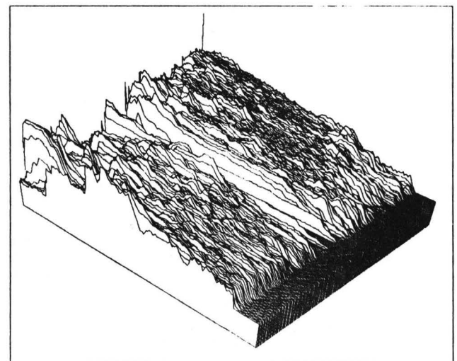
Perspective view of final edge and intensity correlation - NVL
