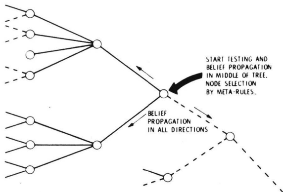
PI DEBUGGING IN A VERY LARGE TREE Figure 3
