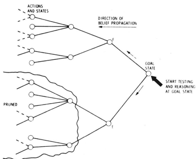
PI TREE FOR IMPLEMENTED EXAMPLE Figure 2
