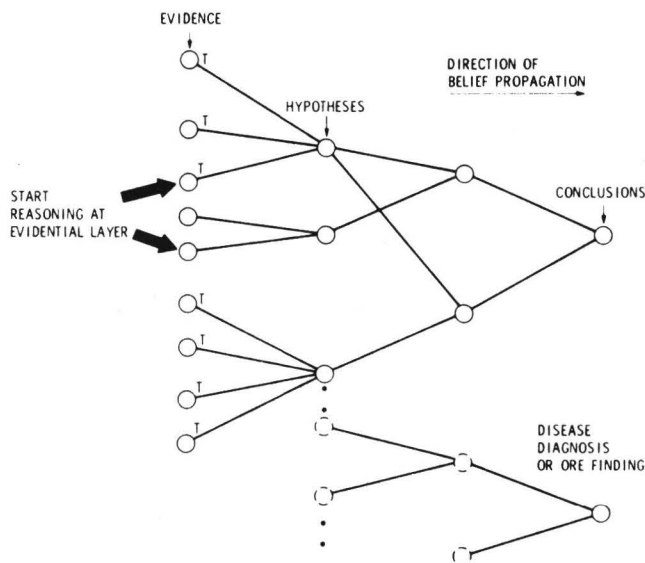
MYCIN/PROSPECTOR TREE Figure 1
