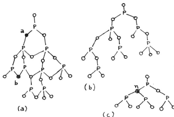
Fig. 2 General P-graphs and hierarchies. (a), (b) are simple; (b) is a hierarchy but (a) is not since there are two paths between " a " and " b ". (c) is not simple, since there are two assertions about " n ".
