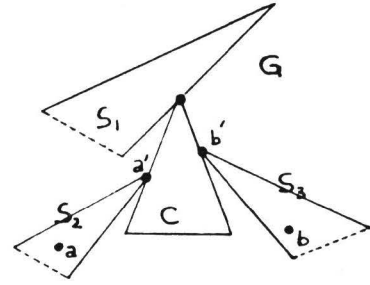
Fig. 5 G is a fully consistent semi-closed P-graph. Subgraphs S_1, S_2, S_3 are semi-closed, and C closed. a' and b' belong to the same closed subgraph C , so P(a', b') and D(a', b') are used. b and b' belong to a smaller semi-closed subgraph, thus the algorithms can be applied recursively to determine whether G \vdash b = b' . Thus if G \vdash b = b' , then if P(a', b') = \text{"yes"} the algorithm yields "yes" for ?[a part-of b].
