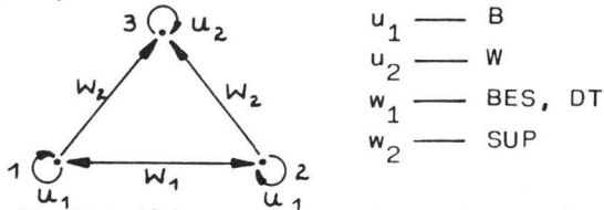
Fig. 2: Ascribing colours to nodes and arcs of fig. 1
