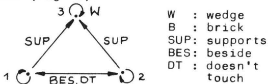
Fig. 1: Labelled graph describing an arch
