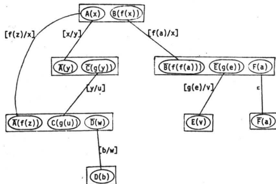
Figure 1: A CIG for clauses \{A(x) B(f(x)), A(y) C(g(y)), D(b), A(f(z)) C(g(u)) D(w), B(f(f(a))) E(g(e)) F(a), E(v), F(a)\} .
