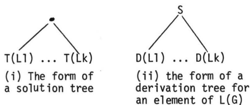
Figure 7: Forms of solution trees and derivation trees for L(G) .
