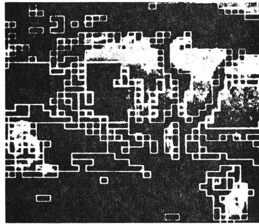
Figure 12. Landscape Scene Partitioned by "Region Color Contrast." Similarity Criterion = |\bar{r}_{ai} - \bar{r}_{bi}| + |\bar{g}_{ai} - \bar{g}_{bi}| + |\bar{b}_{ai} - \bar{b}_{bi}|
