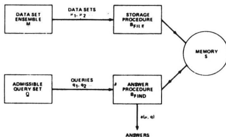
Figure 1. Block Diagram Model of a Question-Answering System.
