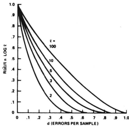
Figure 3. Normalized Rate-Distortion Function for L -Category Classification.
