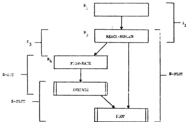
Figure 3. Data Path with Program and Function
