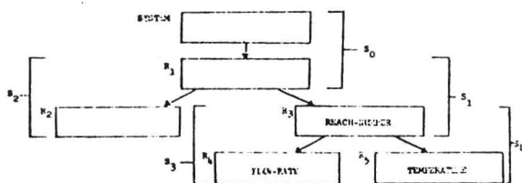
Figure 2a. Example Set Structure
