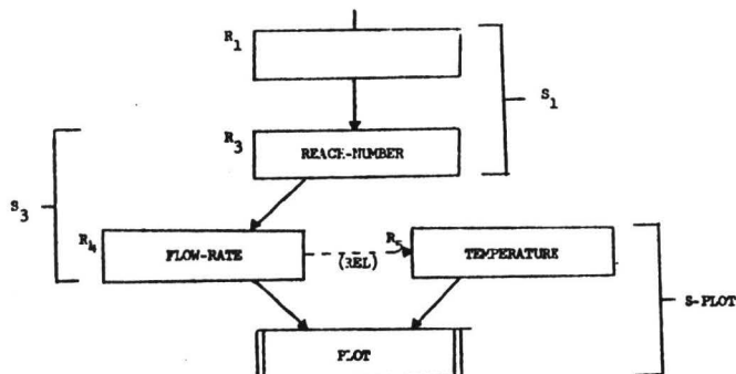
Figure 4a. Path with Specific Function
