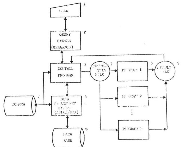
Figure 1. GPLAN Framework
