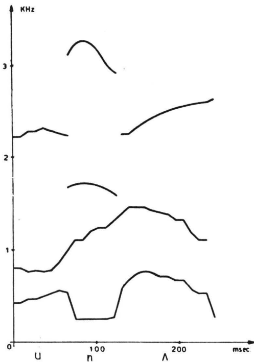
Fig. 3a - Formants of the syllable 'una'
