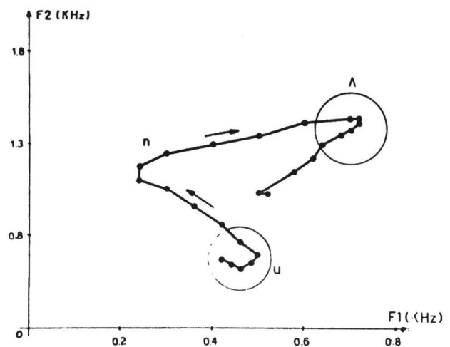
Fig. 3b - Parametric representation of F_1 and F_2
