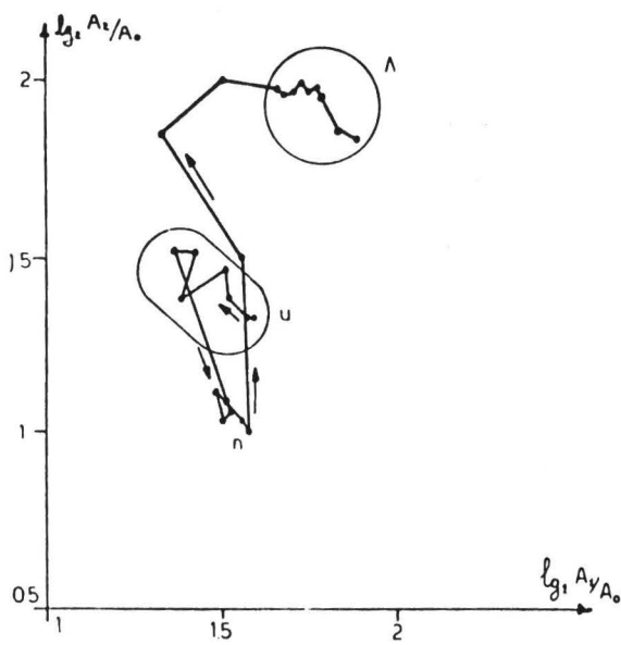
Fig. 3d - Parametric representation of A_1 A_2
