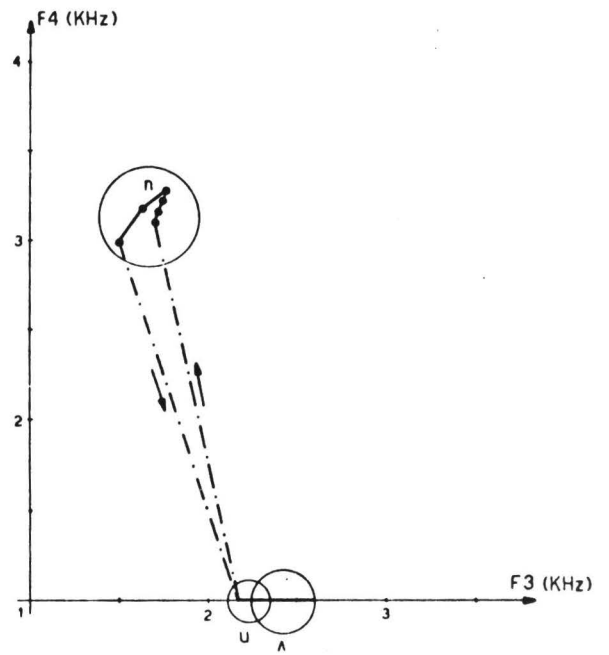
Fig. 3e - Parametric representation of F_3 F_4
