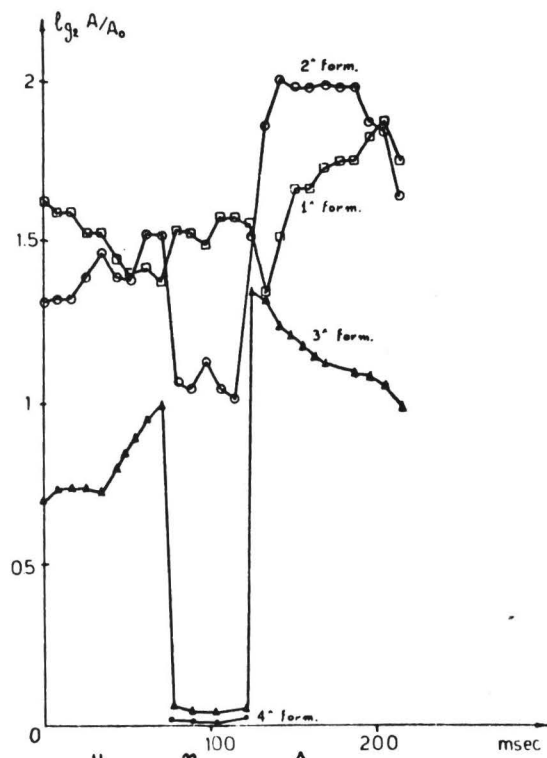
Fig. 3c - Formant amplitudes of the syllable "una"
