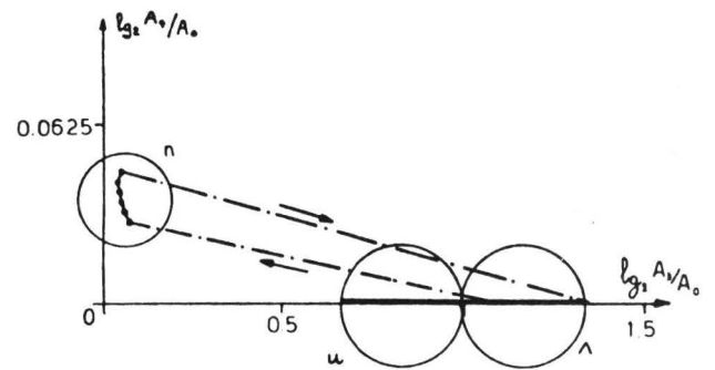
Fig. 3f - Parametric representation of A_3 A_4
