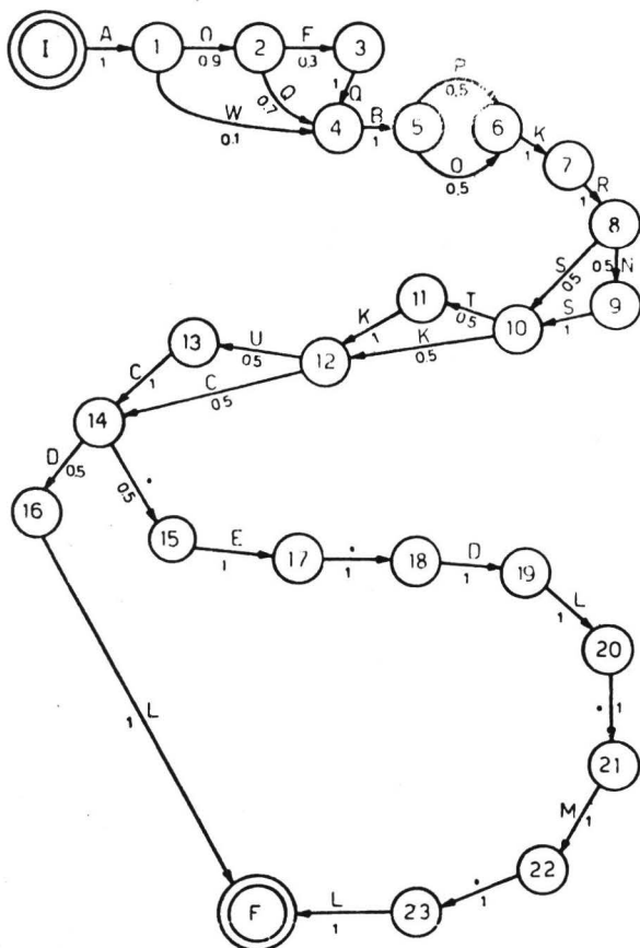
Fig. 4 - SFSA of the syllable "unw".
