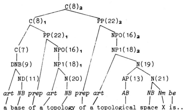
Fig. 3. The numbers given in parentheses with the nonterminal symbols are the production rule numbers. Subscripts are used for references.
