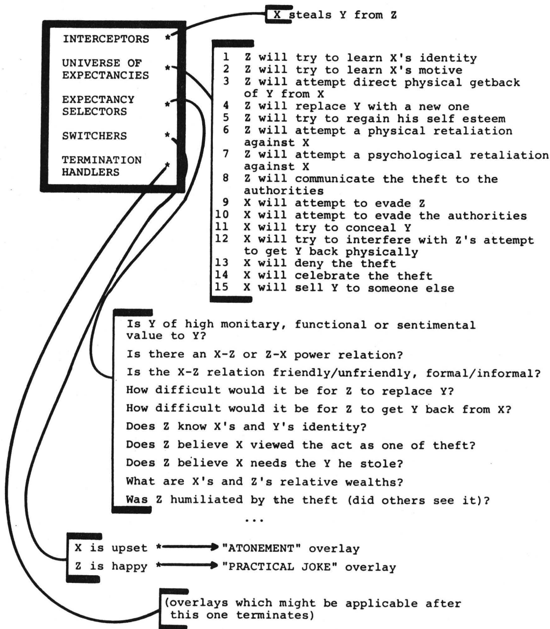
Figure 1. The action overlay relating to thefts.
