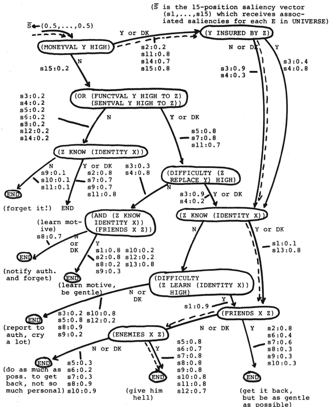
Figure 3. Selector function discrimination net for the theft overlay of Fig. 2.
