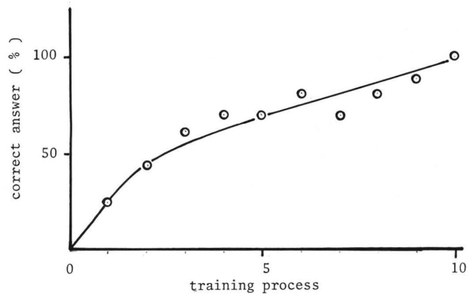
Fig.11 Learning process
