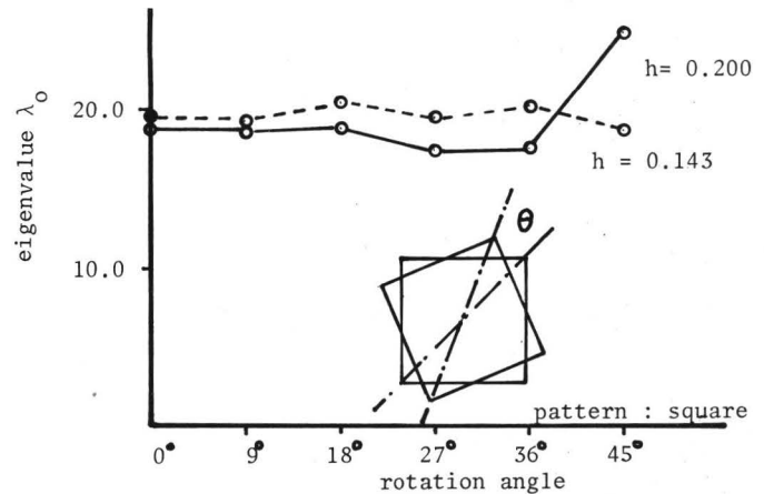
Fig.5 Rotated pattern and its eigenvalue
