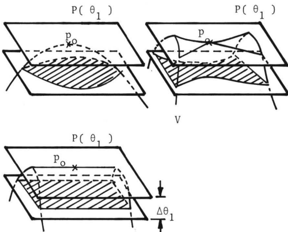
Fig.2 Dupin's indicatrix
