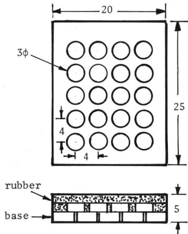
Fig. 8 The artificial tactile sense with multi-elements
