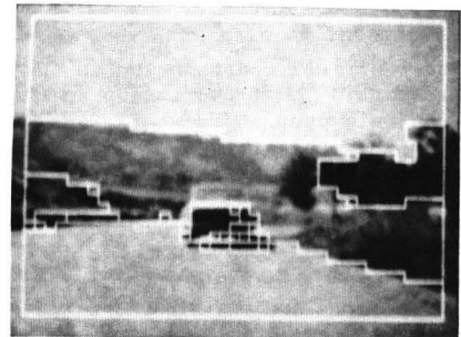
(A-4) Result of merging regions down to 30 regions using weakest boundary first algorithm and non-semantics boundary strength evaluation. Note that the top of the car is melted into the roadside vegetation.
