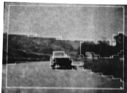
(A-7) Final grouping of regions based on the interpretation assigned to them by the world model. Regions whose meaning was assigned with confidence less than 10 are not mergable. They occur usually on the real boundary between two regions.
