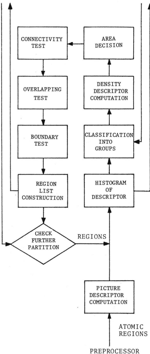
Fig.6 Detailed Block Diagram of Homogeneity Analyzer
