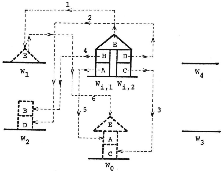
Fig.6 Transitions of states ( job sequence : 1,2,---,6 )
