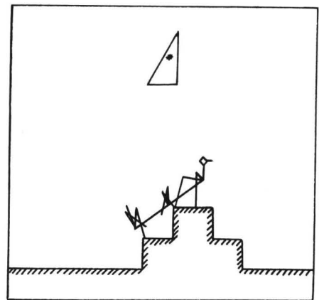
Fig. 10. Climbing over a complicated obstacle.
