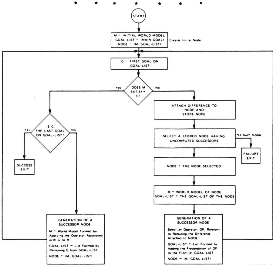
FIGURE 2 FLOW CHART FOR STRIPS
