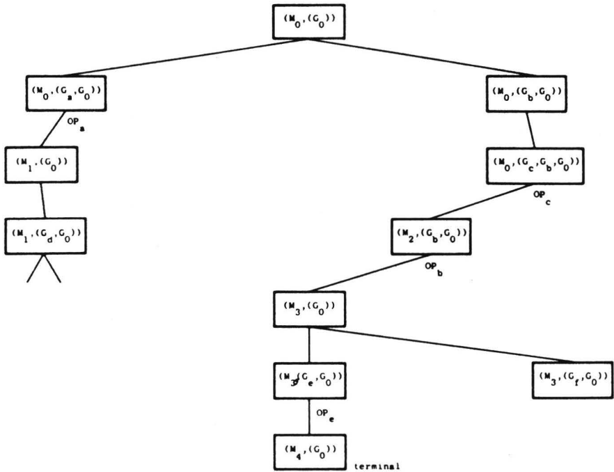
FIGURE 1 A TYPICAL STRIPS SEARCH TREE
