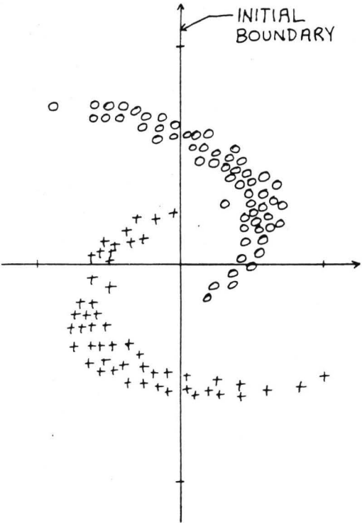
Figure 4. Classification of nonlinearly separable data.
