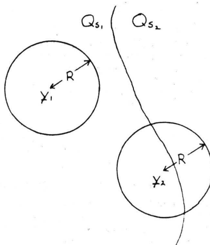
Figure 1. Asymptotic fixed neighborhood decision rule.
