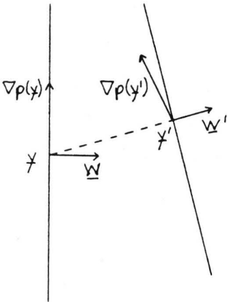
Figure 3. Perturbation of a stationary boundary.
