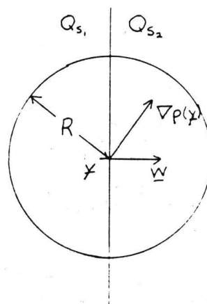
Figure 2. Classification of a boundary point.
