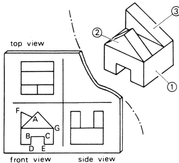
Fig. 4 Example of a three-view drawing and its three-dimensional configuration.
