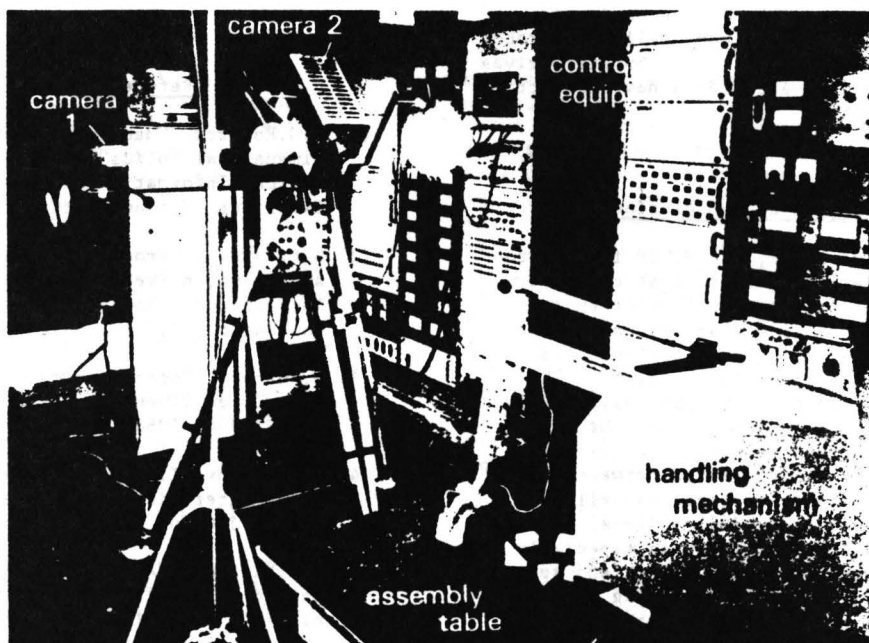
Fig. 2 General view of the intelligent robot.
