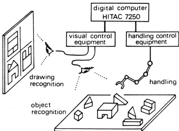
Fig. 1 Outline of the intelligent robot.
