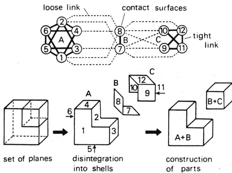
Fig. 5 Recognition process of individual parts from the integrated three-dimensional structure.
