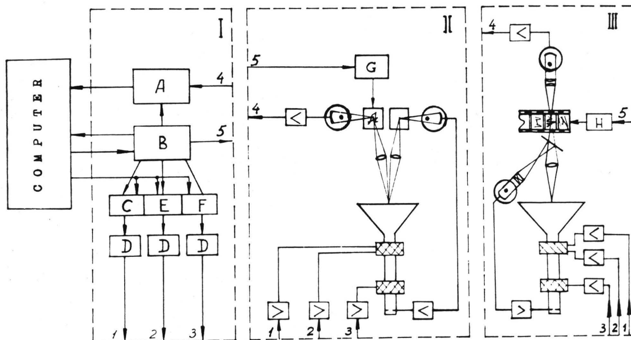
Fig.2 A Block Diagram of the Scanner Units and Connections with the Local Control Unit
