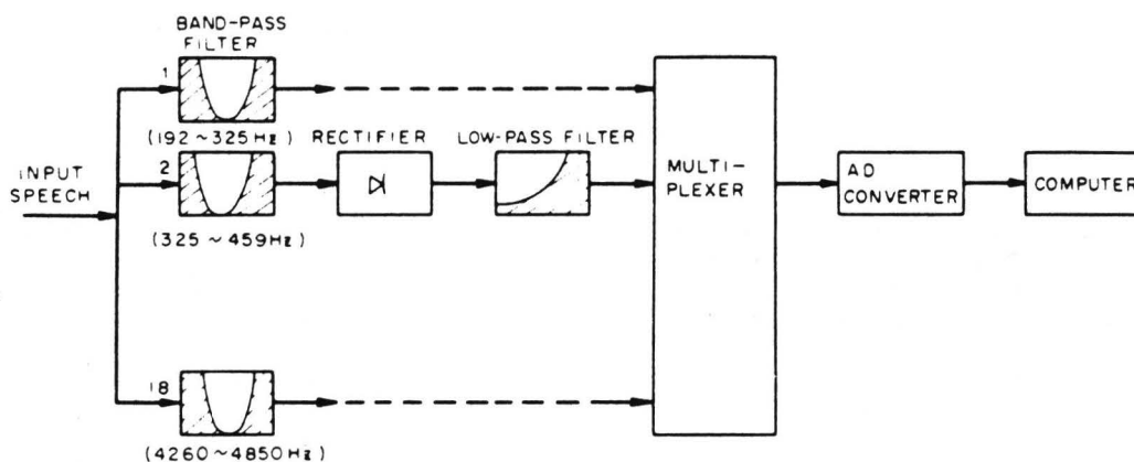
Fig.3 Frequency analysis and computer input system
