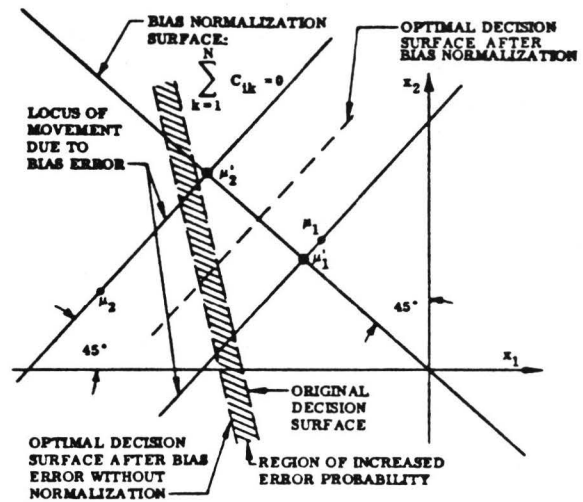
Fig. 7 Normalization for Uniform Bias Error
