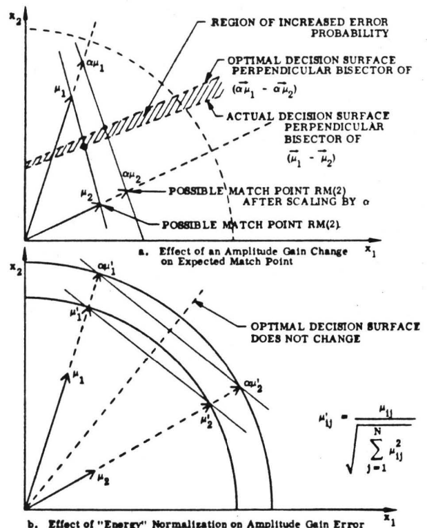
Fig. 6 Normalization for Uniform Amplitude Gain Error
