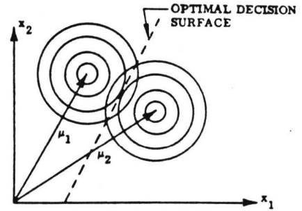
a. Case of Spherically Symmetric Noise Which Is Identical and Uncorrelated for All Variables ( \sigma_1 = \sigma_j ; \rho_{ij} = 0 )
