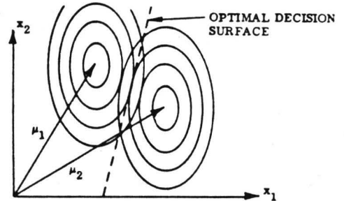
b. Case of Ellipsoidally Symmetric Noise Which Is Not Identical but Is Uncorrelated for All Variables ( \sigma_1 \neq \sigma_j ; \rho_{ij} = 0 )
