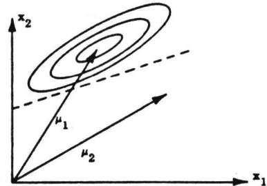
c. Case of Ellipsoidally Symmetric Noise Which Is Not Identical and May Be Correlated for All Variables ( \sigma_1 \neq \sigma_j ; \rho_{ij} \neq 0 )
