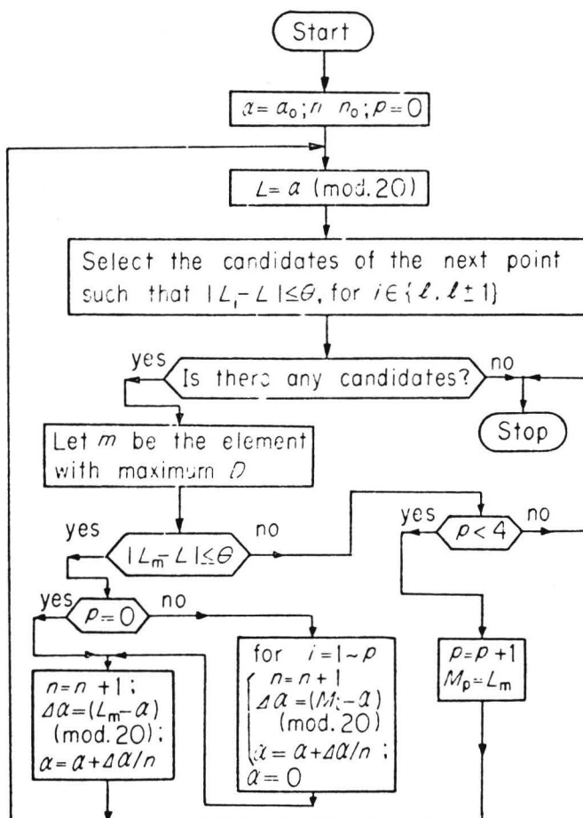
Fig.7. Flow chart of the tracking
