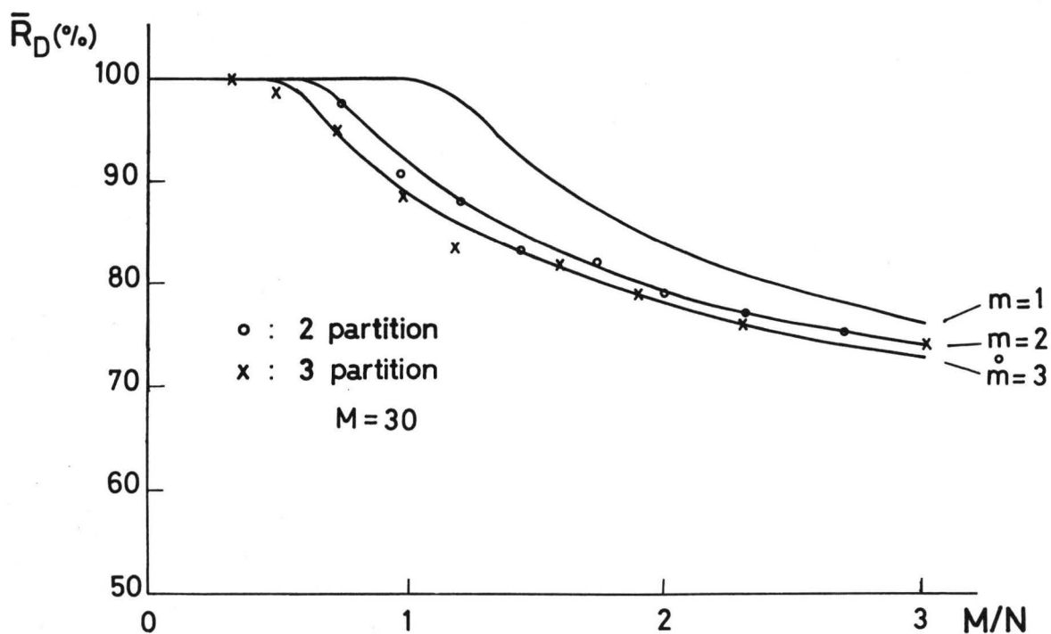
Fig.3 The relation between \bar{R}_D and M/N
