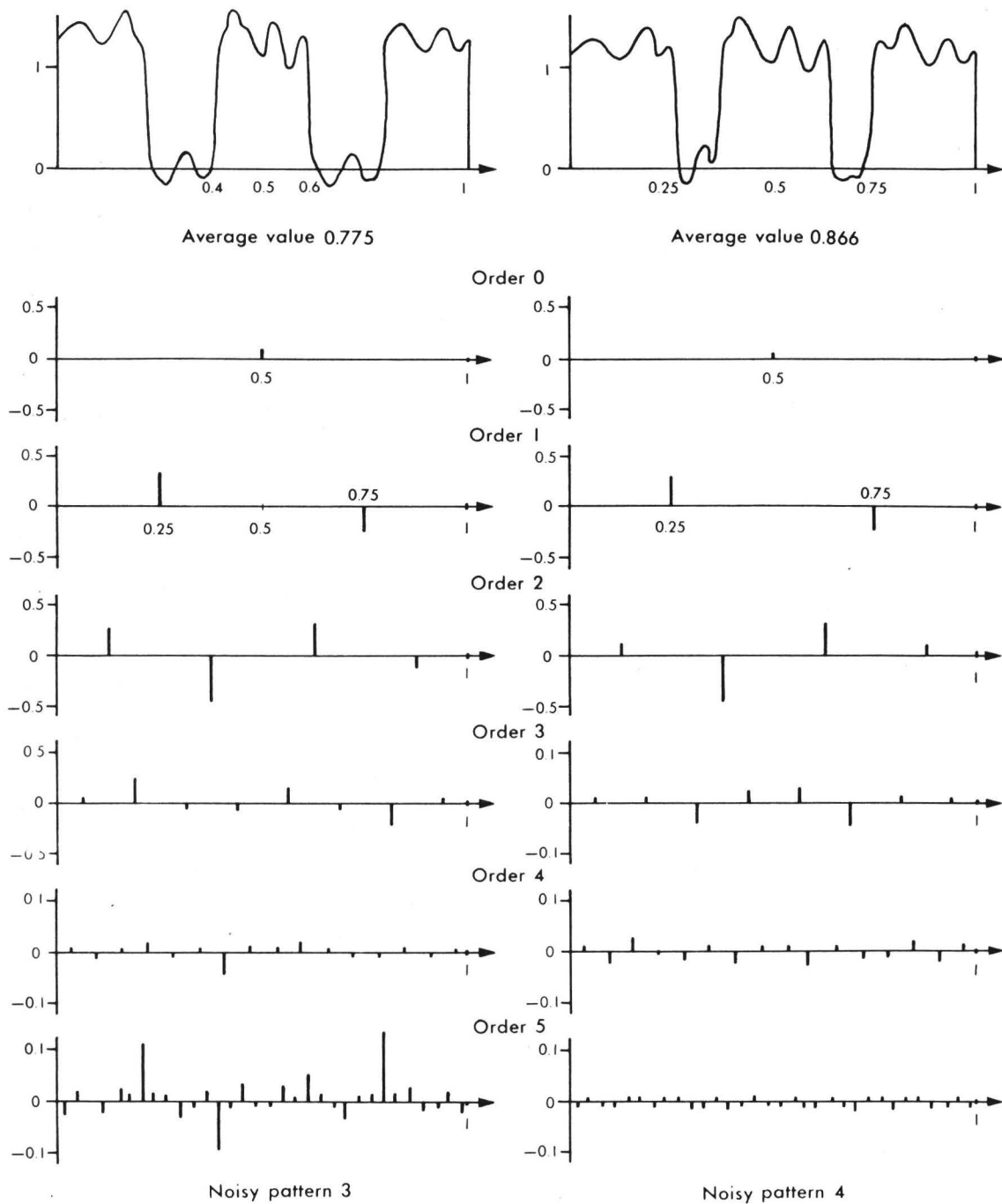
Fig. 9 - Analysis by HAAR functions
