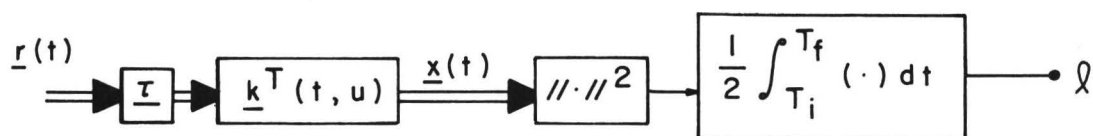
(b) Array Energy Detector Structure
