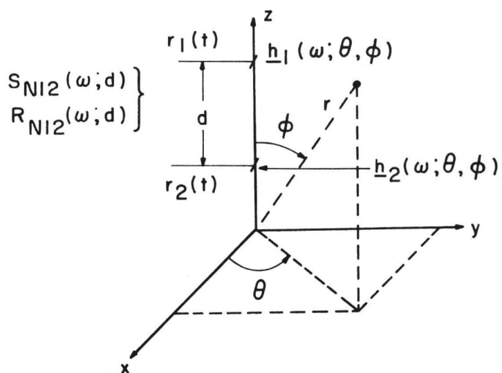
FIGURE 3. SPACE-TIME CORRELATION GEOMETRY.
