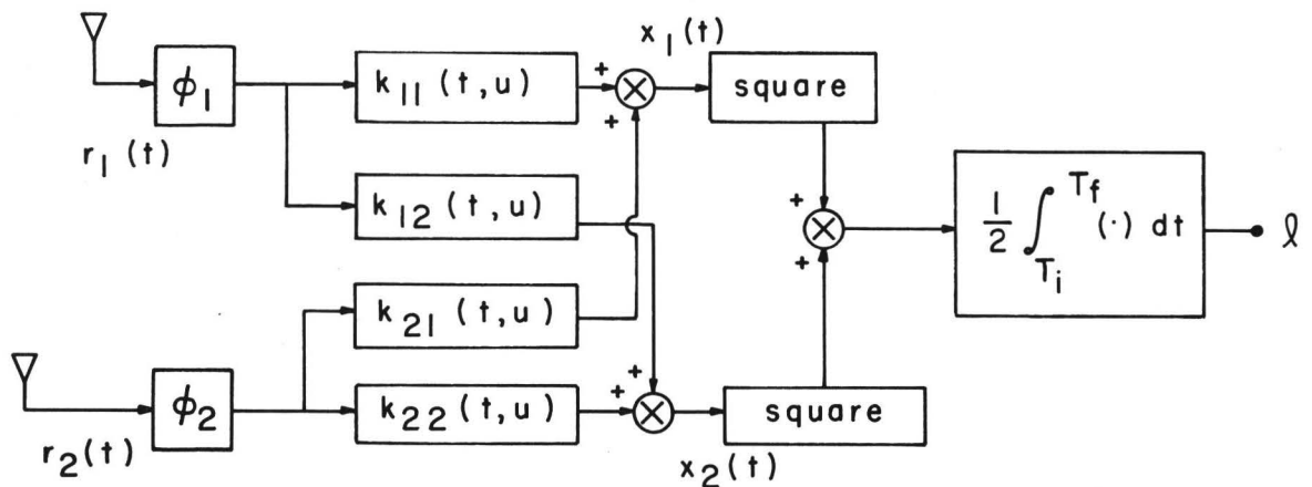
(b) Array Energy Detector Structure
