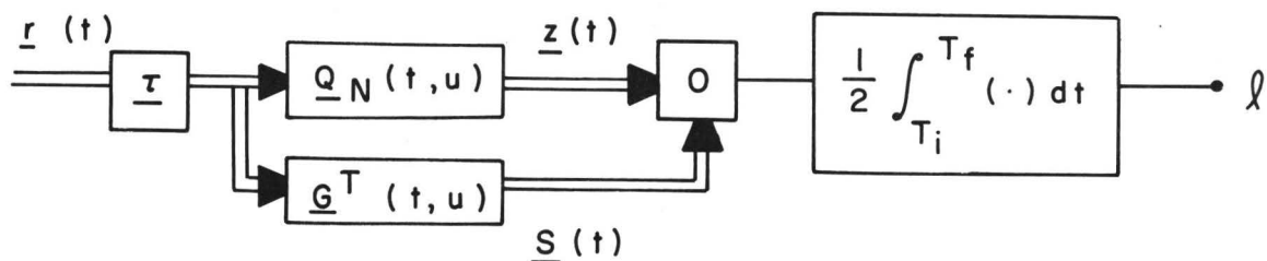
(a) Phaser / Weighter / Combiner - Estimator - Correlator Structure
