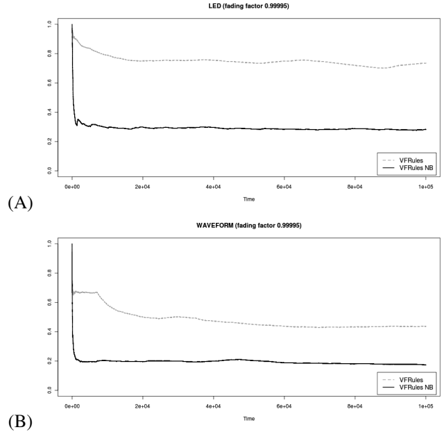
Figure 1: Prequential error of VFDR MC and VFDR NB in LED (A), and Waveform (B).
