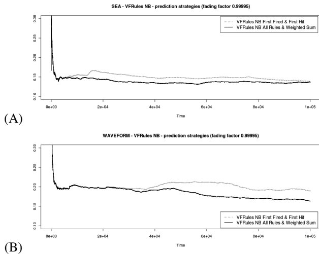
Figure 2: Error-rate curves of \text{VFDR}_{NB} with different learning and prediction strategies in SEA (A), and Waveform (B) datasets.
